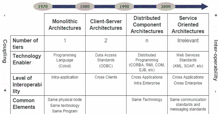
Figure 1. Software architectures evolution 1
