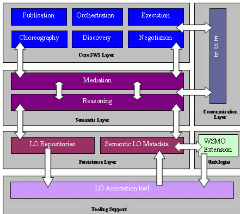
Figure 3. Layered architecture
